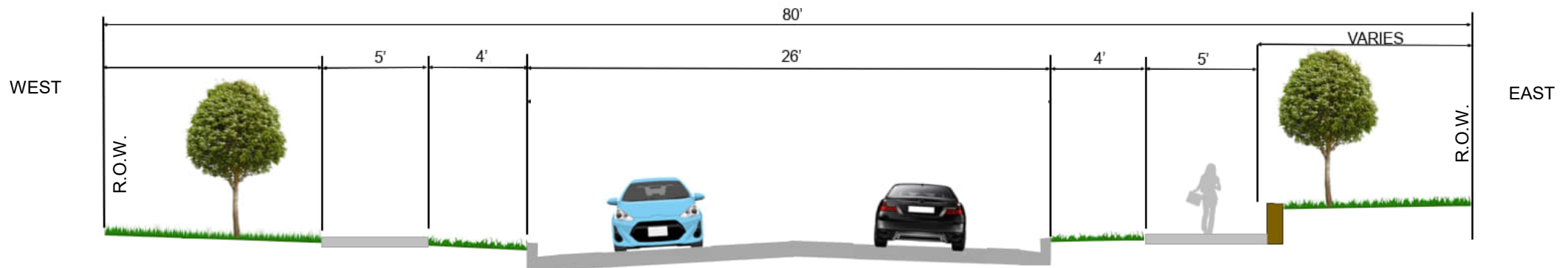
Proposed N. Gilbert Street Southern Typical Section
